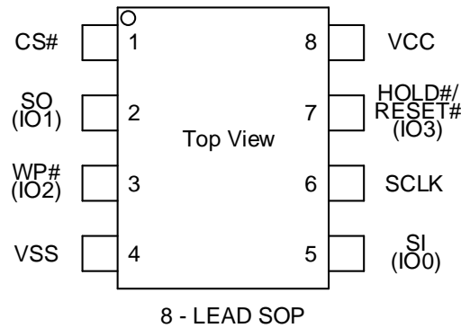
Figure 3 Connection Diagram for SOP8 package
