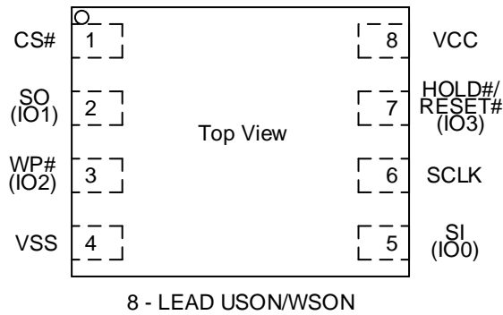
Figure 2 Connection Diagram for USON8/WSON8 package
