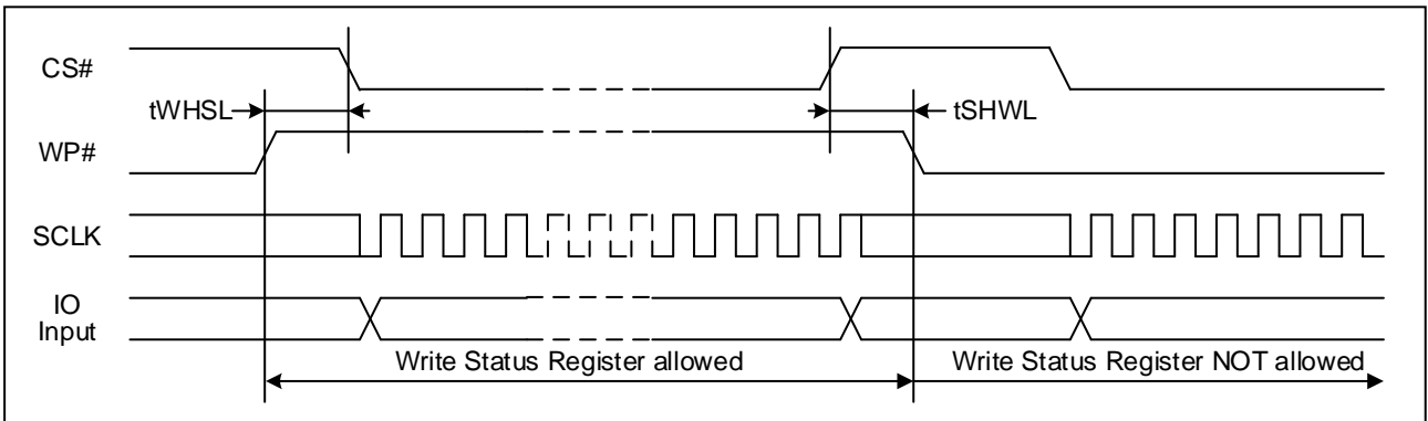
Figure 50. WP# Timing
