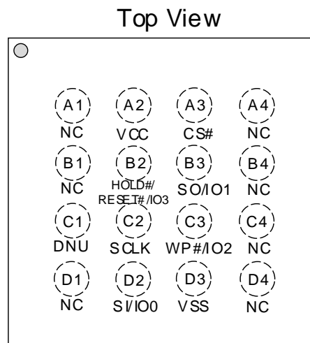
WLCSP (4-4 ball array)
