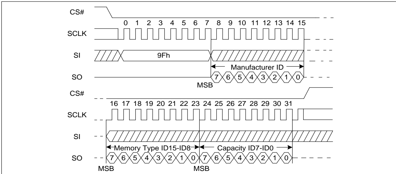
Figure 29. Read Identification ID Sequence Diagram
