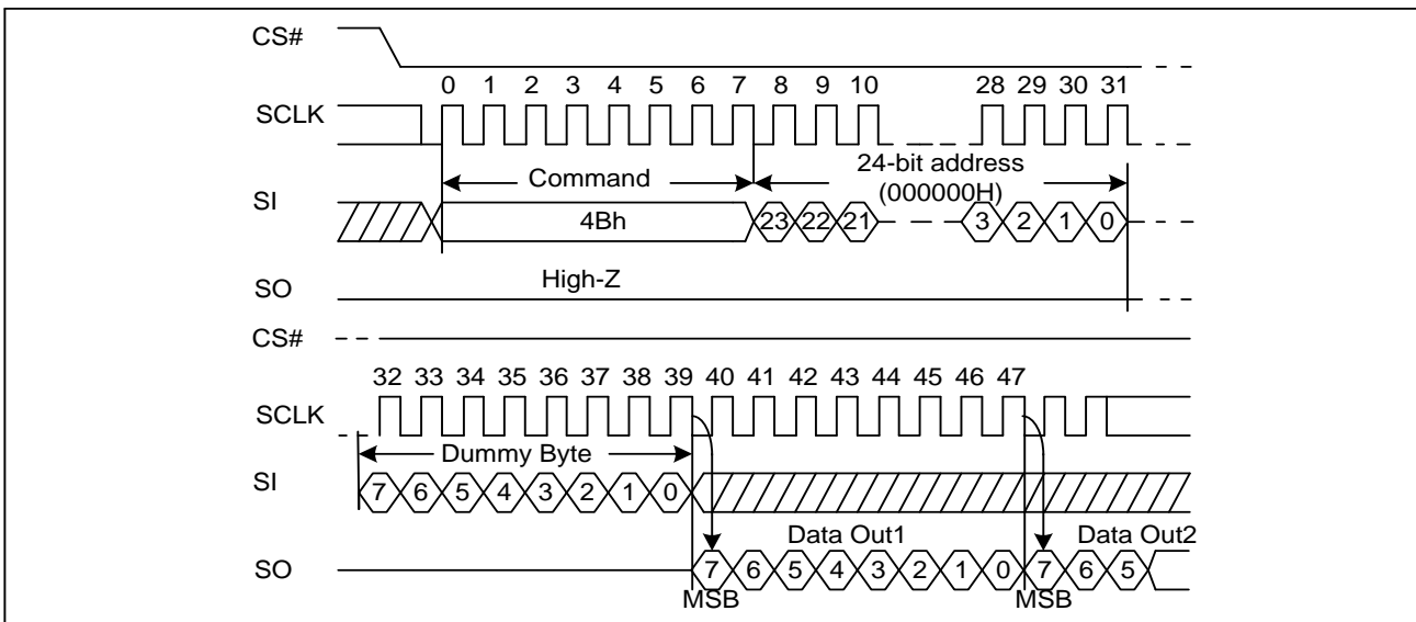
Figure 30. Read Unique ID Sequence Diagram
