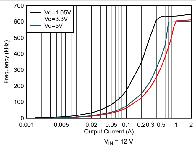
图 5-8. TPS562201 Switching Frequency vs Output Current V_{IN} = 12\text{ V}
