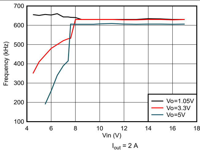
图 5-7. TPS562208 Switching Frequency vs Input Voltage I_{out} = 2\text{ A}
