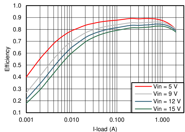
图 5-10. TPS562201 V_{OUT} = 1.5\text{ V} Efficiency, L = 2.2\text{ }\mu\text{H}
