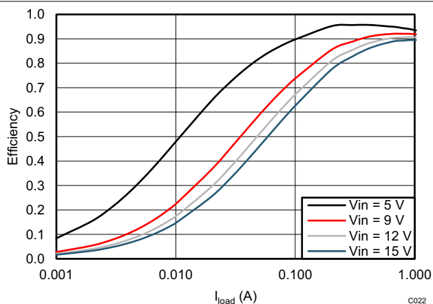
图 5-17. TPS562208 V_{OUT} = 3.3 V Efficiency, L = 2.2 \mu H
