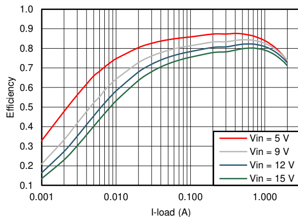
图 5-9. TPS562201 V_{OUT} = 1.05\text{ V} Efficiency, L = 2.2\text{ }\mu\text{H}
